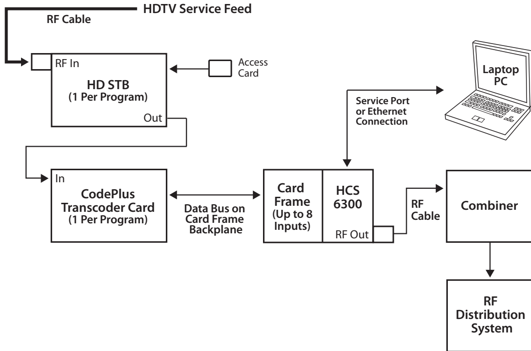
Typical Setup Flow Chart for HCS6300
