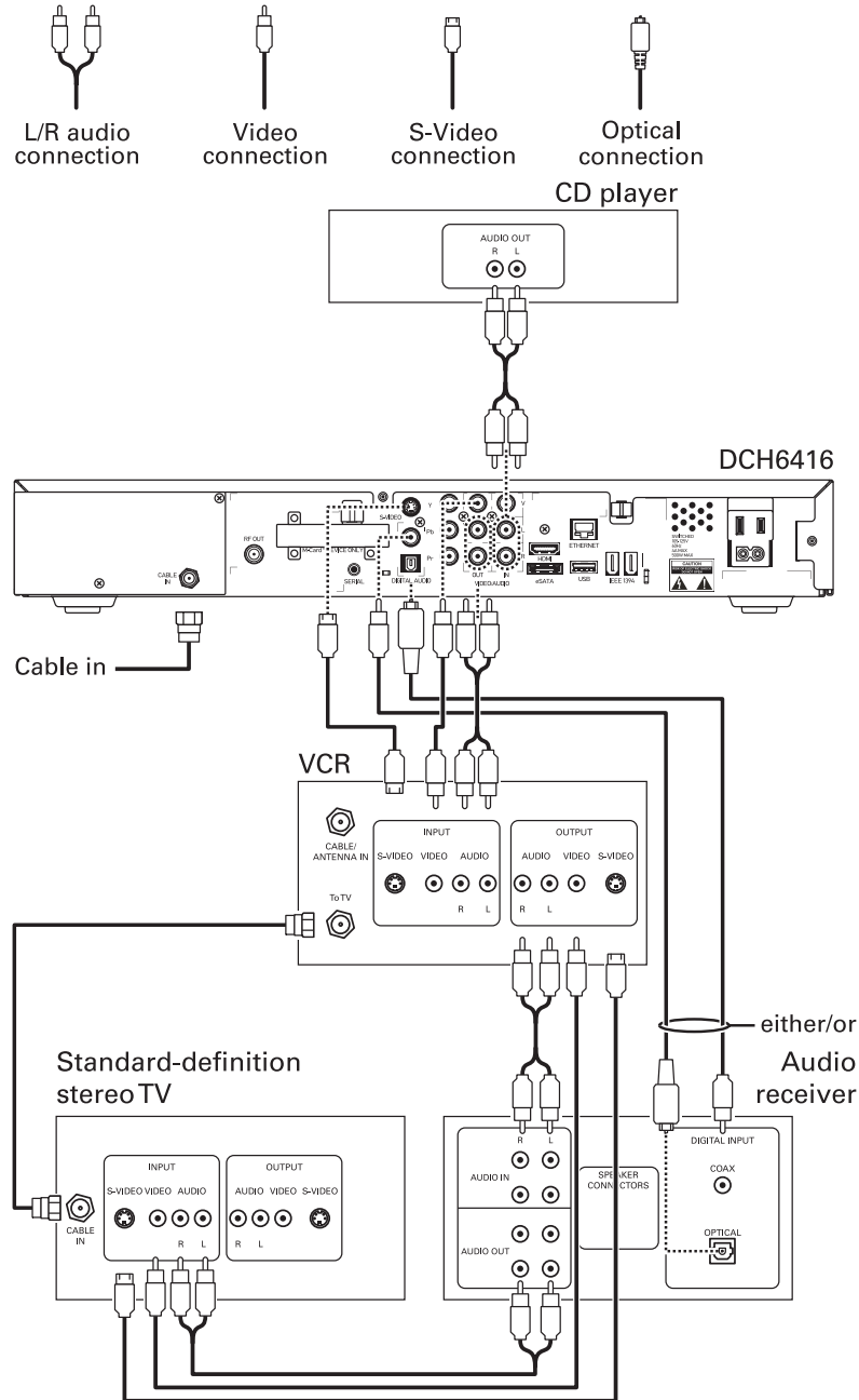
Figure 3-4 Cabling an audio receiver
