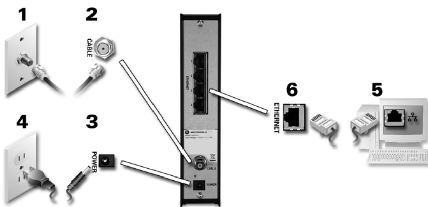
Figure 1 – Cabling the SBG941
