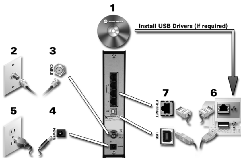
Figure 2 – Cabling the SBG941U
