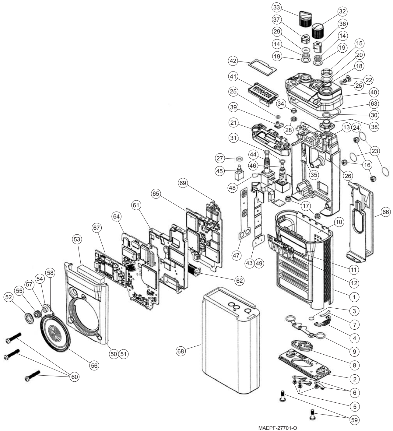
Figure 7-1. SSE 5000 Exploded View
