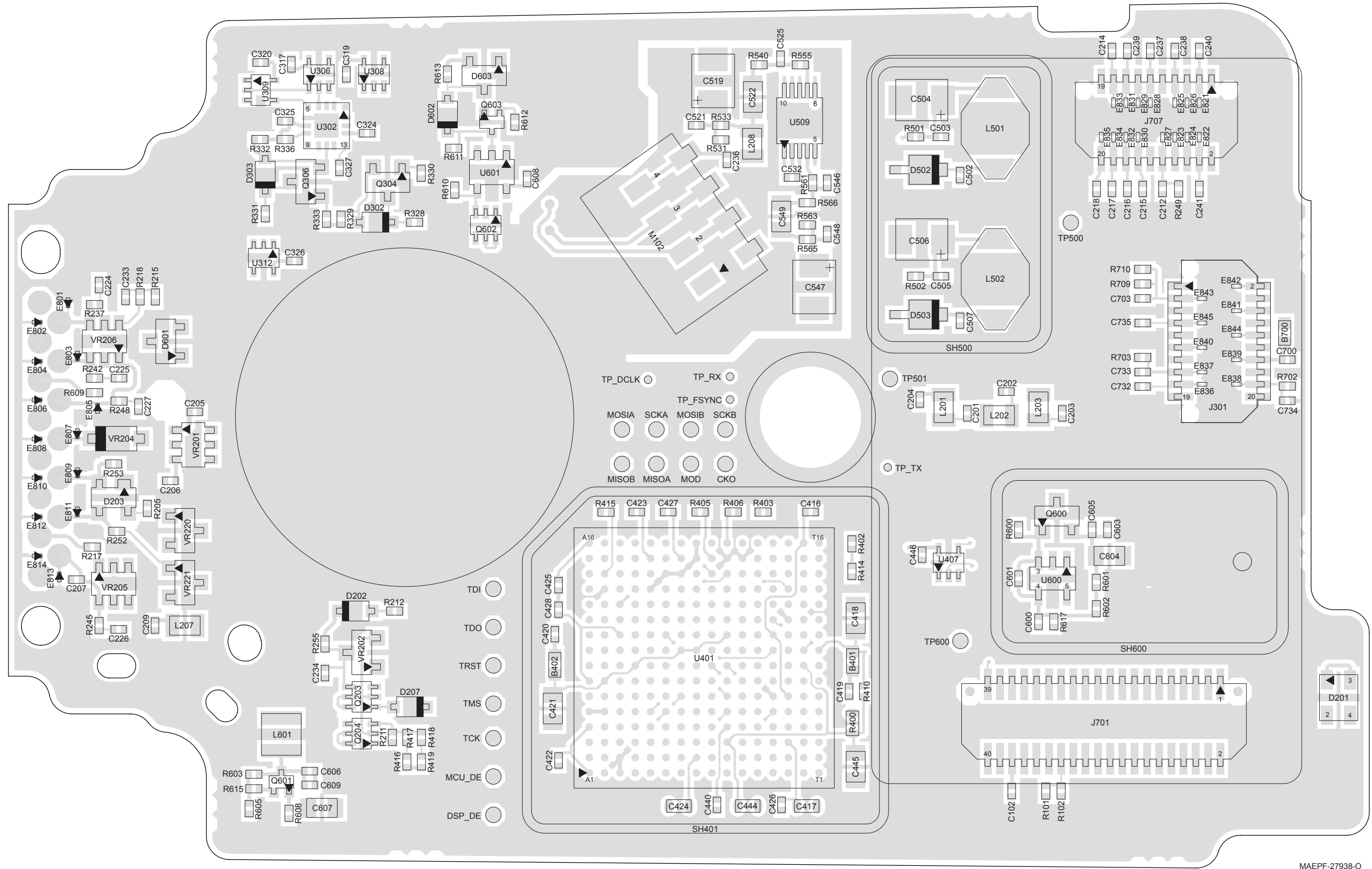
Figure 12-21. NCN6186_ VOCON Board Layout—Side 1
