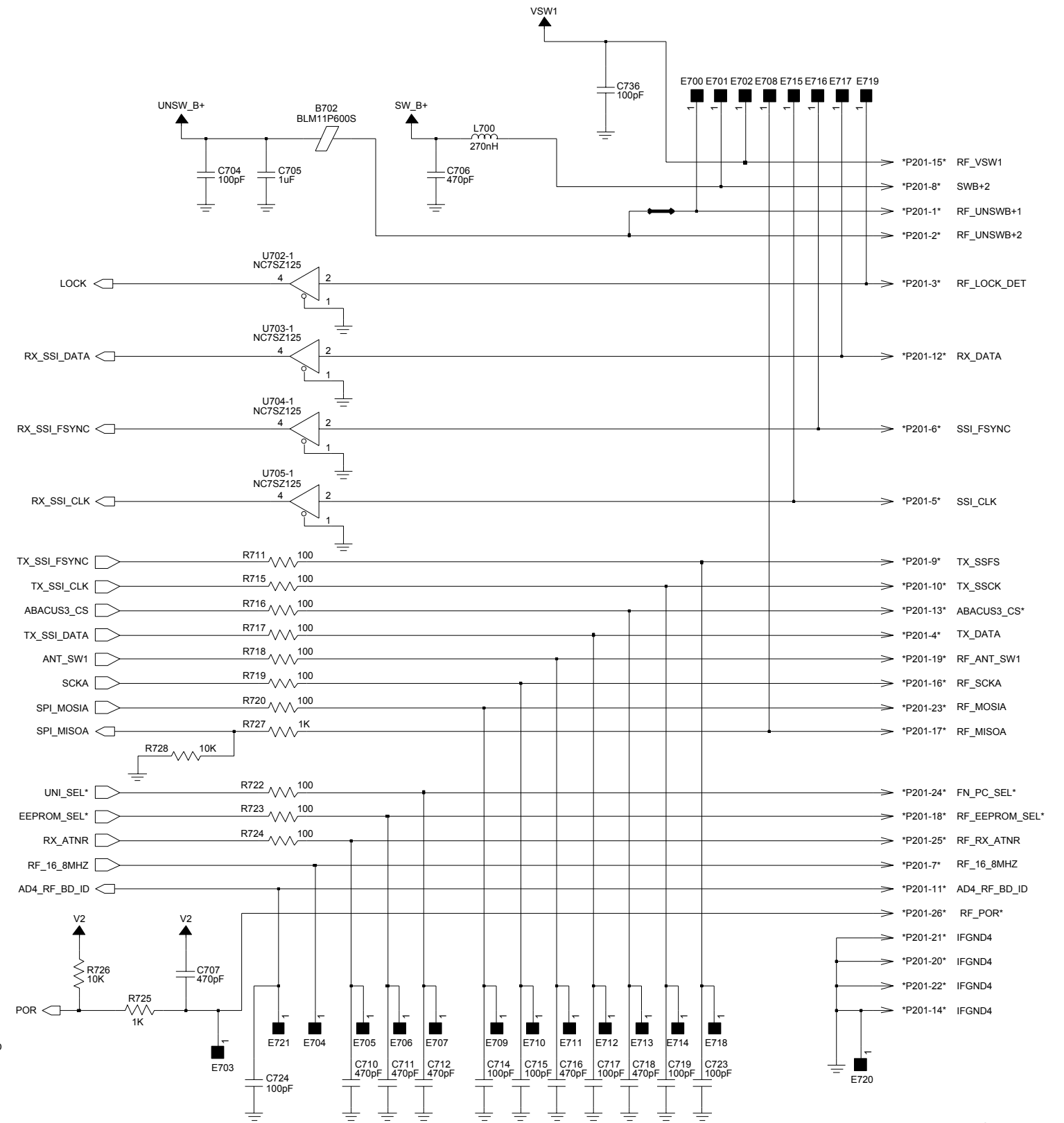
Figure 12-19. NCN6186_VOCON Display-RF Interface
