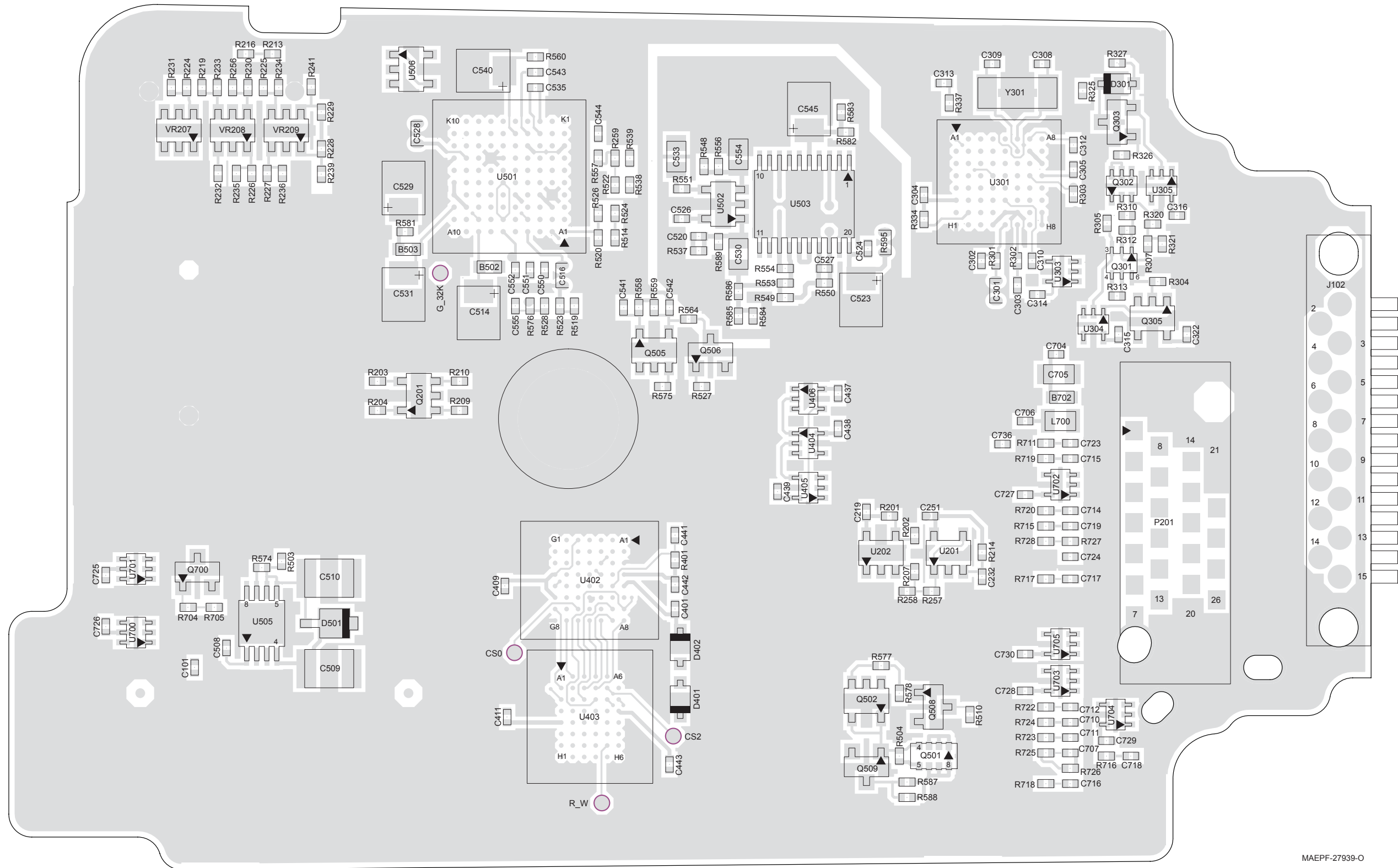
Figure 12-22. NCN6186_ VOCON Board Layout—Side 2
