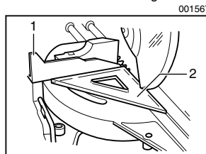
1. Guide fence 2. Triangular rule
