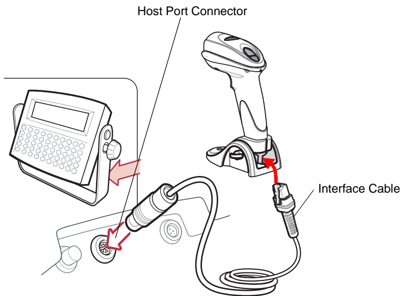
Figure 11-2 Scanner Emulation Connection for Scanner with Base
