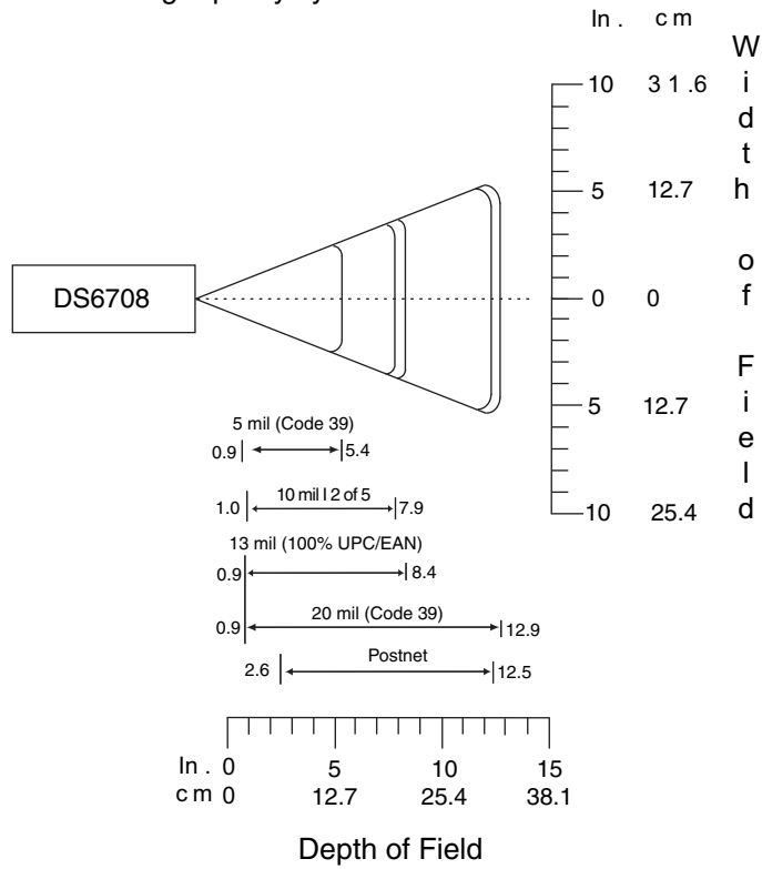
Figure 2-16 Symbol DS6708 Digital Scanner Decode Zone for 1D Bar Codes
