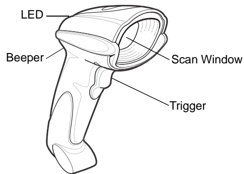
Figure 1-1 Symbol DS6708 Digital Scanner
