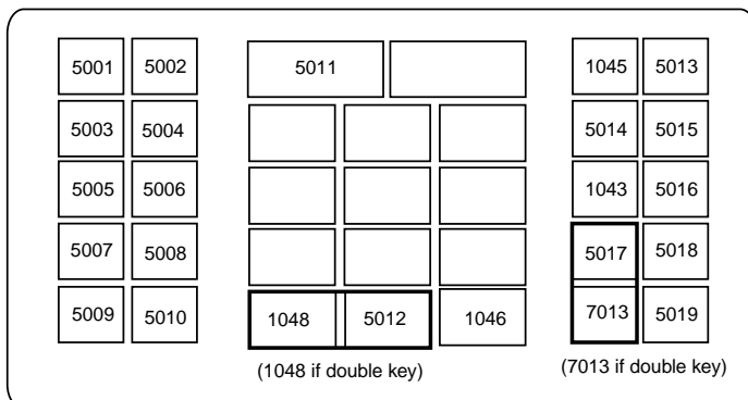
Figure 10-5 NCR 7052 32-Key
