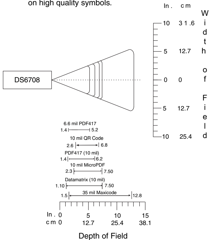
Figure 2-17 Symbol DS6708 Digital Scanner Decode Zone for 2D Bar Codes
