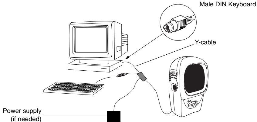
Figure 5-1. Keyboard Wedge Connection with Y-cable
