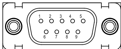
Figure 8-1 Symbol MS3207 Connector
