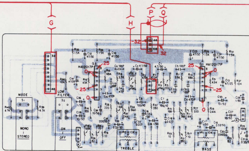
TONE CONTROL Ass'y GWG-141
