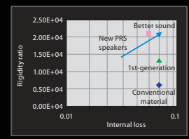
Physical properties of cone materials
