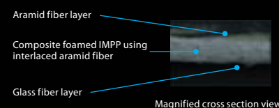
Physical properties of cone materials
