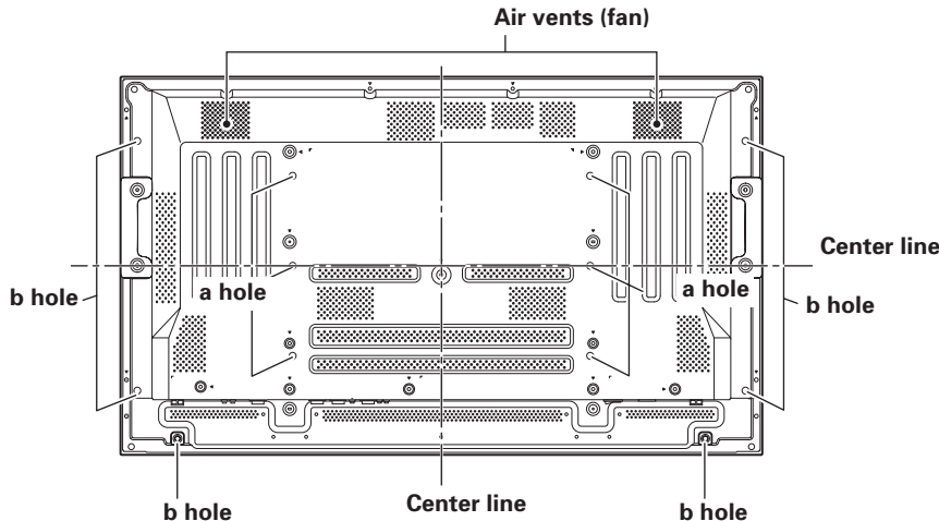
Rear view diagram (PDP-434CMX)
