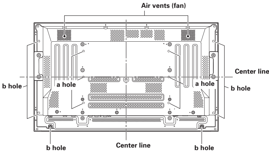
Rear view diagram (PDP-434CMX)
