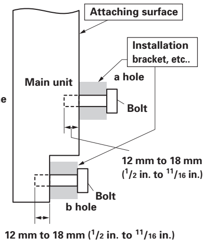
Side view diagram
