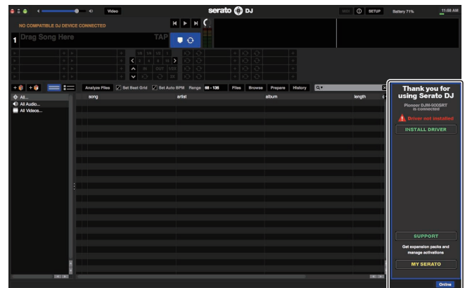
1 License panel
