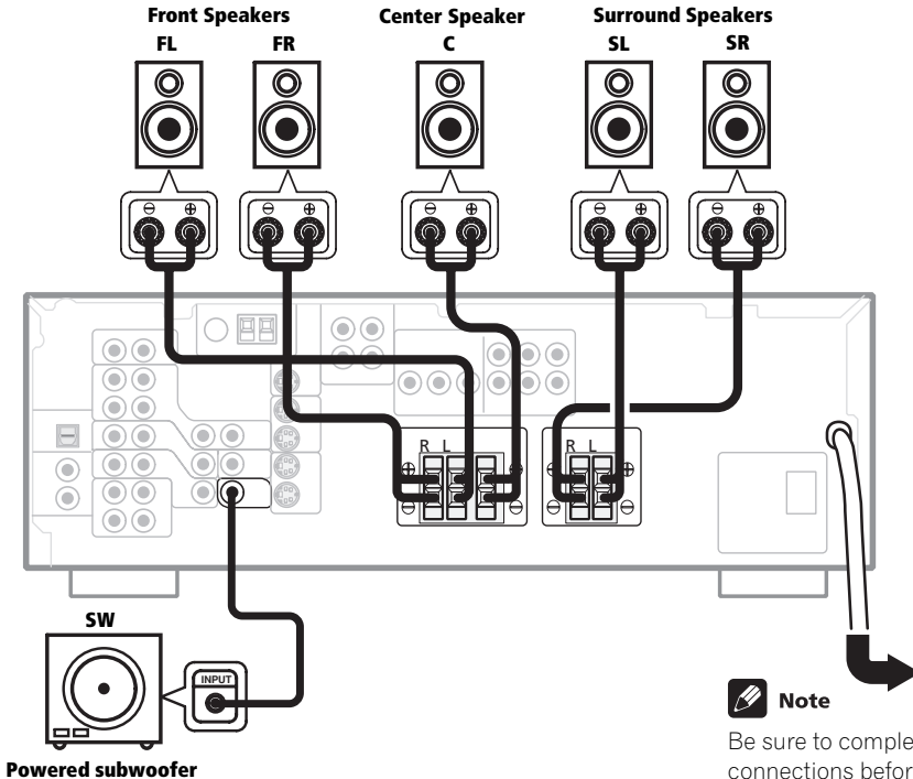
Powered subwoofer
