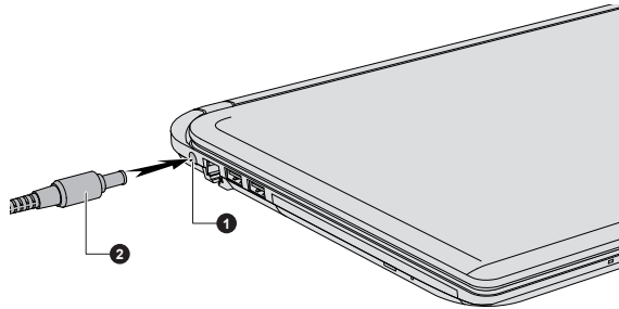
Figure 2-3 Connecting the DC output plug to the computer
