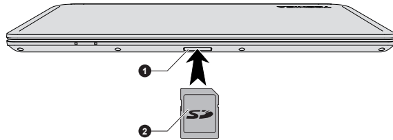
Figure 4-7 Inserting memory media
