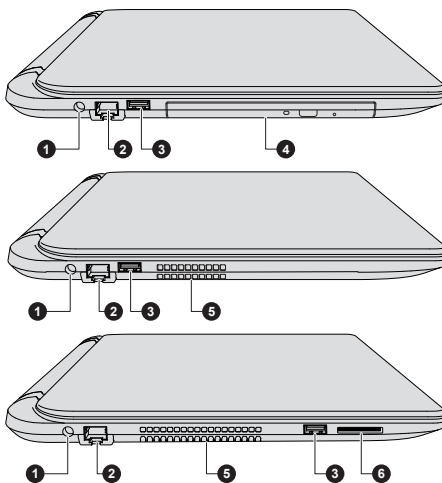
Figure 3-2 The left side of the computer
