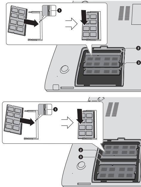
Figure 4-7 Seating the memory module
