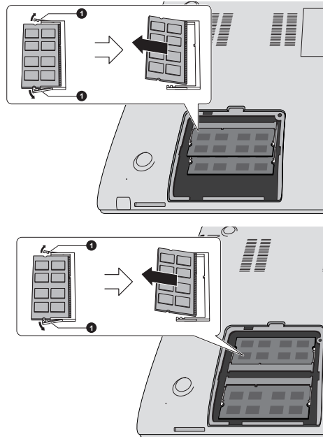
Figure 4-9 Removing the memory module
