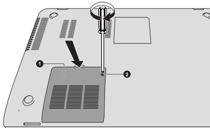
Figure 4-8 Seating the memory module cover
