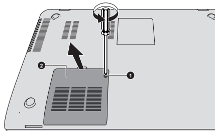
Figure 4-6 Removing the memory module cover
