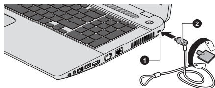
Figure 4-16 Security lock
