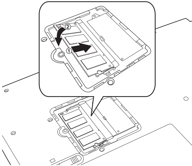
Installing a module
