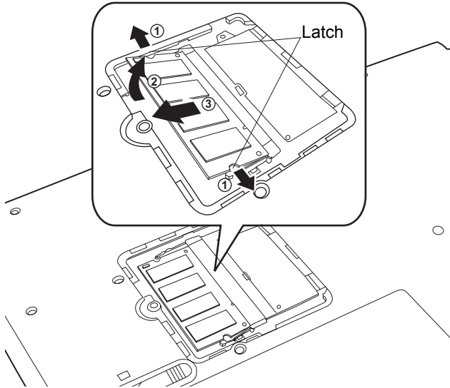
Removing the memory module
