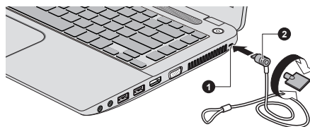
Figure 4-14 Security lock
