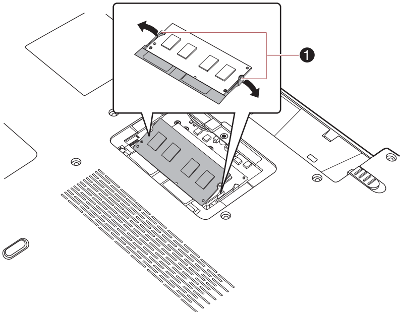
Figure 3-6 Removing the memory module
