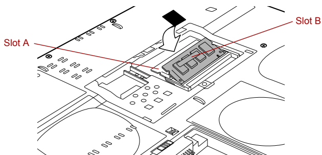
Seating the memory module
