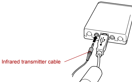
Connecting the infrared transmitter cable
