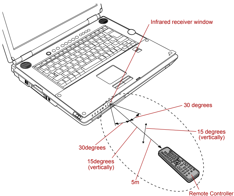
Operational range of the remote control
