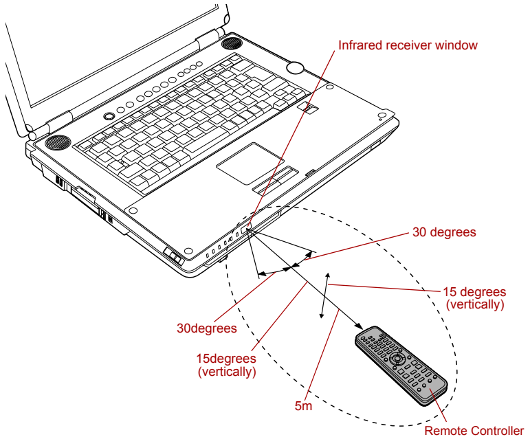
Operational range of the remote control
