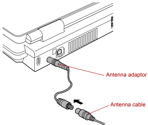
Connecting the antenna cable
