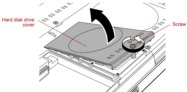
Removing a Hard disk drive cover
