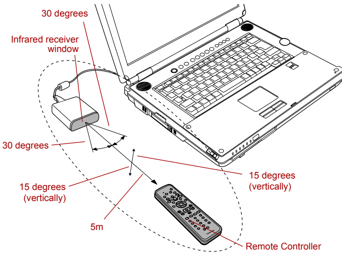
Operational range of the Remote controller
