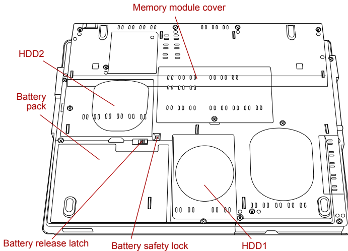
The underside of the computer
