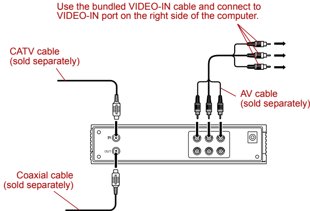
Connection method for the computer and Set-top Box
