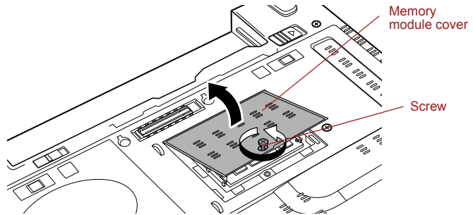
Figure 3-10 Removing the memory module cover
