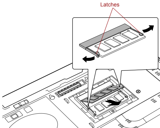
Figure 3-13 Removing the memory module
