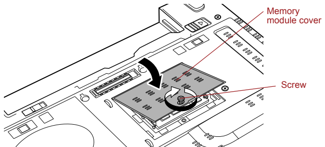
Figure 3-12 Seating the memory module cover
