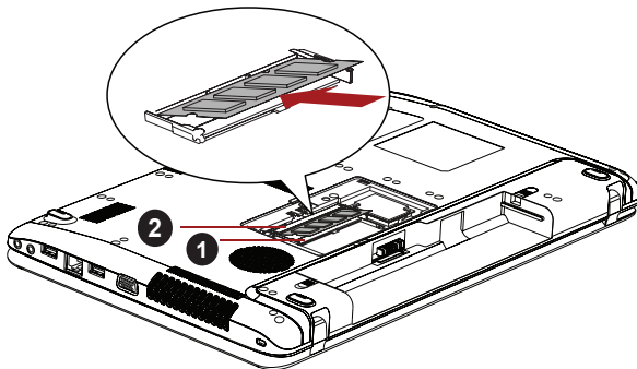
Figure 3-5 Seating the memory module-1
