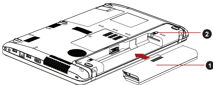
Figure 6-3 Securing the battery pack
