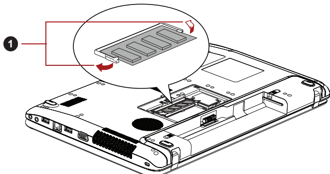
Figure 3-7 Removing the memory module
