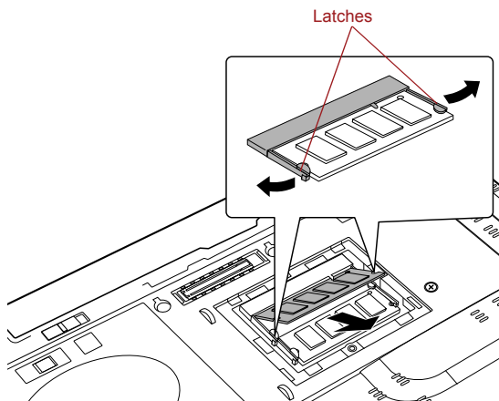
Figure 3-13 Removing the memory module
