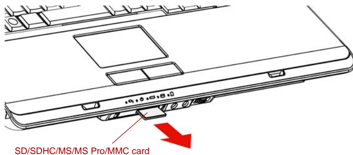
Figure 8-4 Removing the inserted memory card
