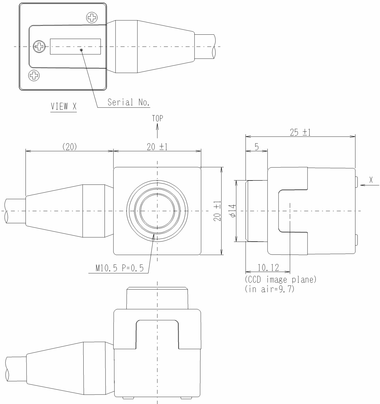
iIS-010 20mm square camera head - external view
