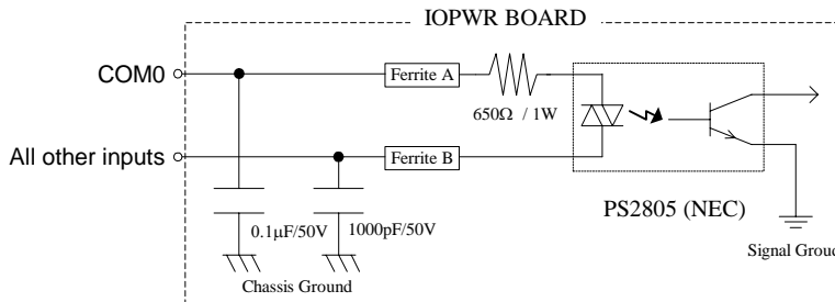
Input circuit
