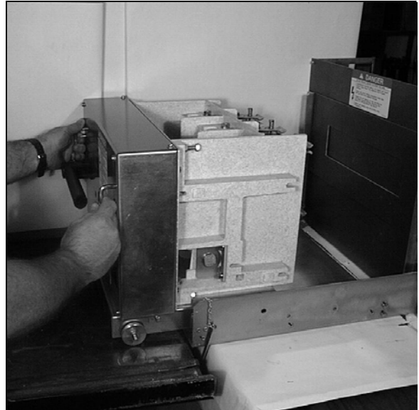
Fig. 19 Inserting Breaker into Cell
