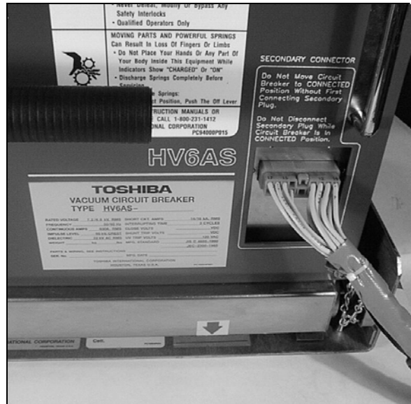
Fig. 21 Control Circuit Plug Connected to Breaker
