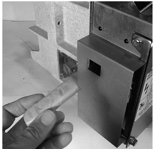
Fig. 29 Removing Plug From UV Trip Device
