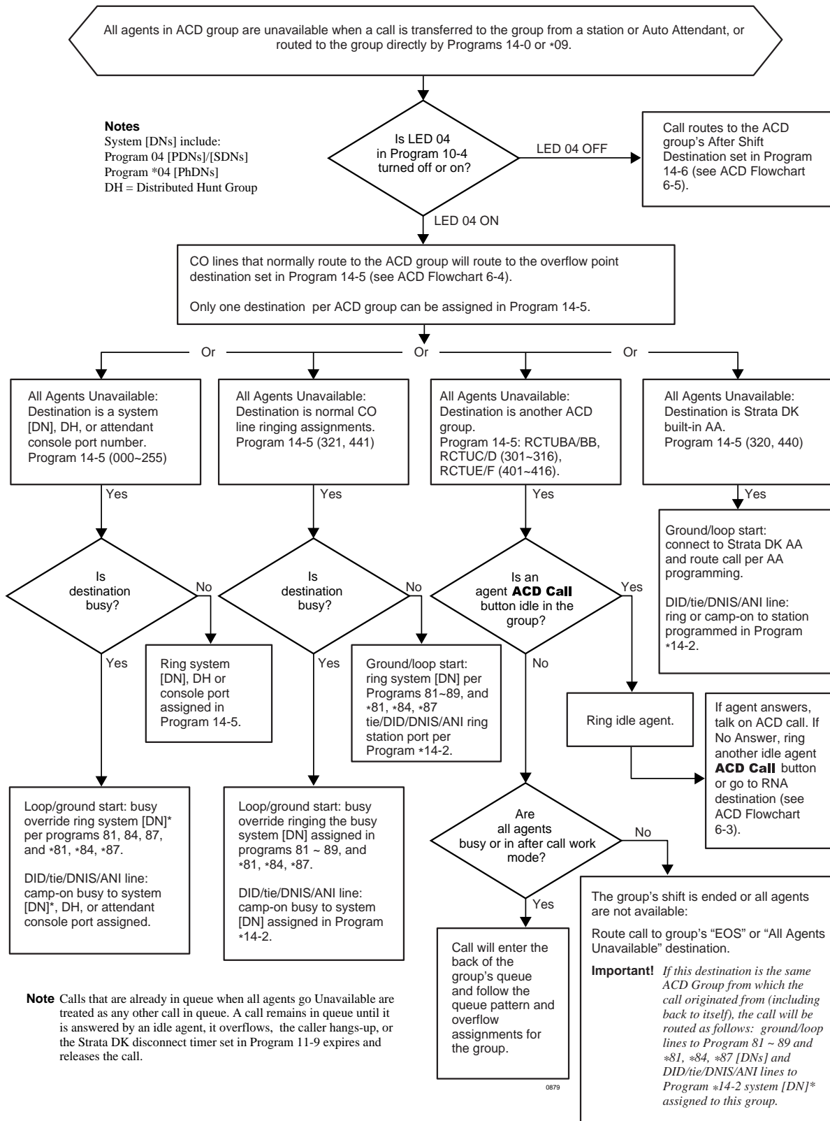
Flowchart 6-6 All Agents Unavailable Operation
