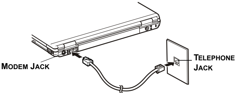
Figure 4-12 Connecting the internal modem
