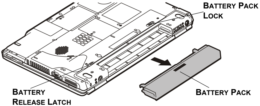
Figure 6-2 Removing the battery pack
