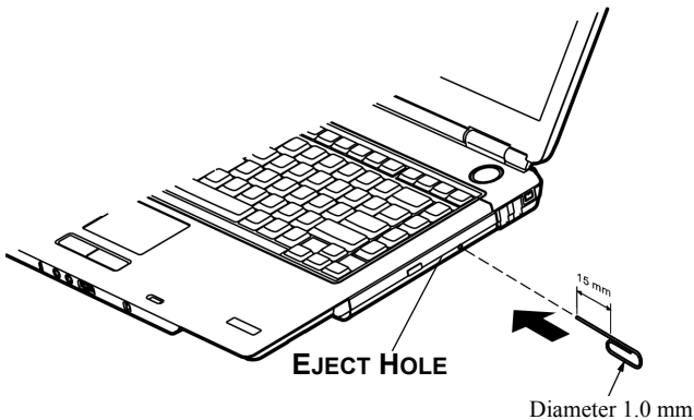
Figure 4-4 Manual release with the eject hole
