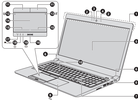
Figure 3-18 The front of the computer with the display panel open (Z50-A)
