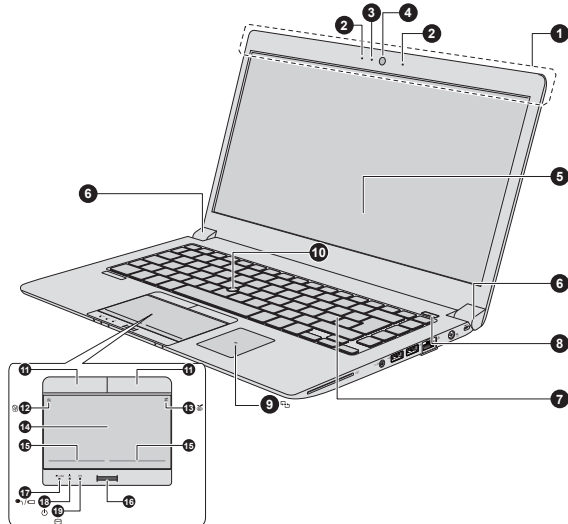
Figure 3-12 The front of the computer with the display panel open (Z40-A)
