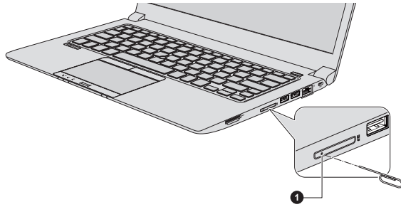
Figure 4-5 Open the SIM card tray with the eject hole (Z40-A)
