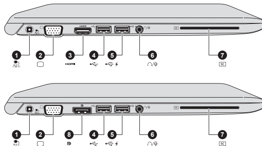
Figure 3-14 The left side of the computer (Z50-A)
