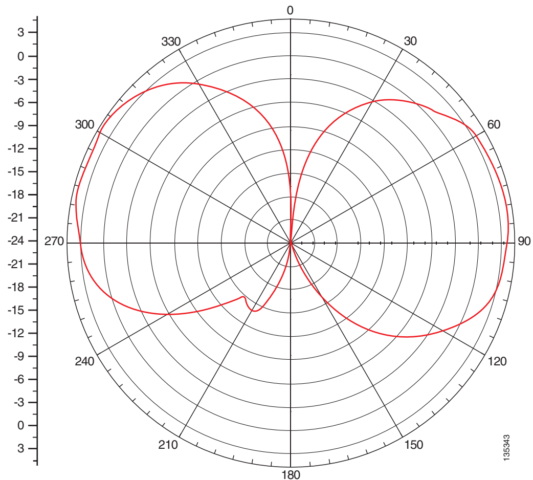
Figure 3 E-Plane Pattern at 2.4- to 2.5-GHz
