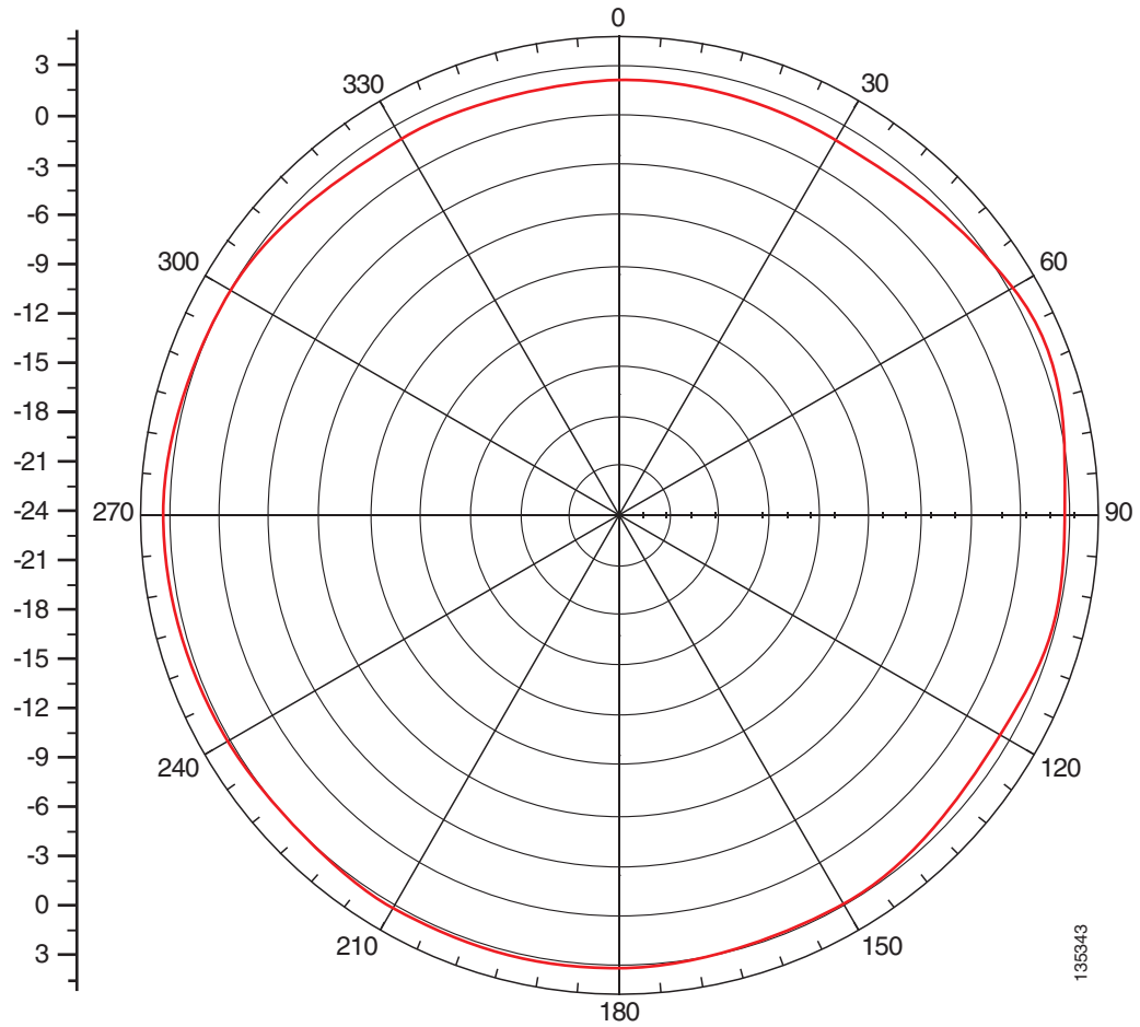
Figure 2 H-Plane Pattern at 2.4- to 2.5-GHz
