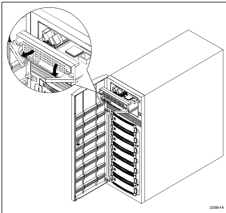
Figure 5-8 Remove controller from top slot
