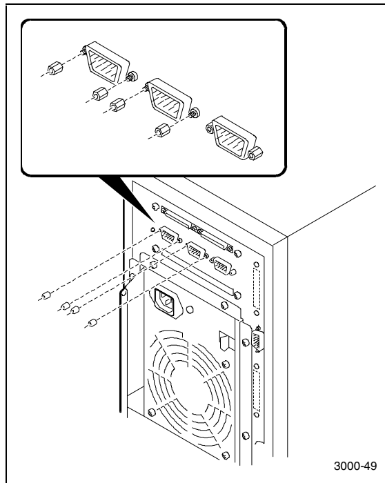
Figure 3-7. Remove standoffs from UPS and external fault connectors
