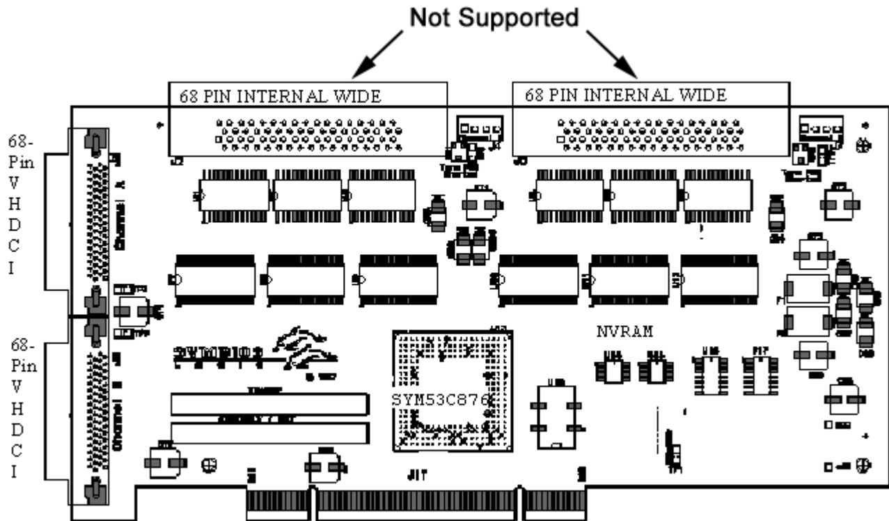
Compaq StorageWorks Dual Channel UWD Library Adapter
