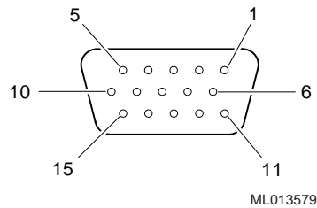
Figure 1-3 VGA Connector Pinouts
