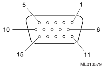
Figure 3-2 VGA Connector Pinouts
