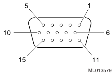
Figure 2-2 VGA Connector Pinouts
