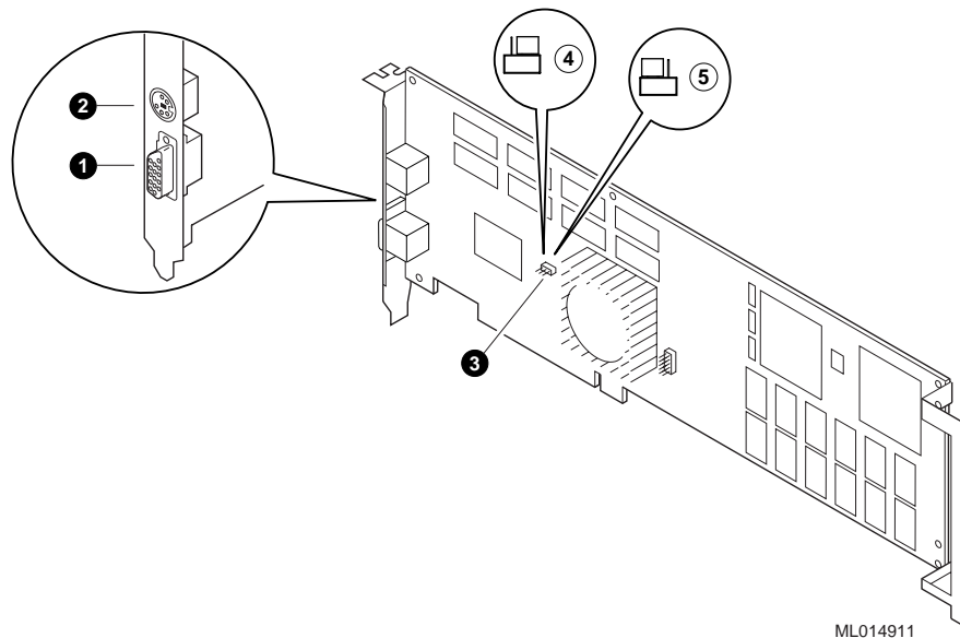
Figure 3-1 PowerStorm 350 PCI Graphics Controller
