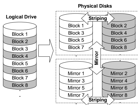
Figure 1 - 6 RAID (0+1)
