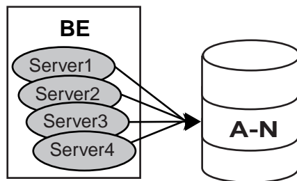
Figure 1–17 Concurrent Servers
