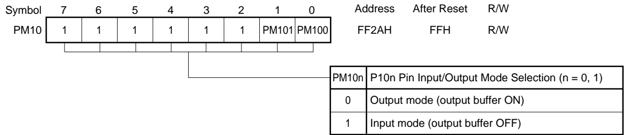
Figure 6-7. Port Mode Register 10 Format
