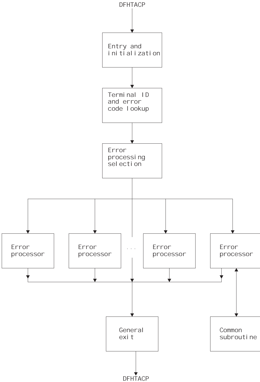
Figure 18. Overview of the sample terminal error program (DFHTACP)
