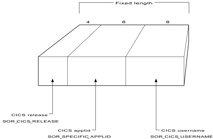
Figure 58. Format of the start-of-run record
