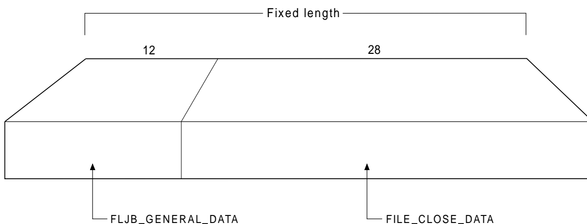
Figure 65. Layout of record written for file-close record types
