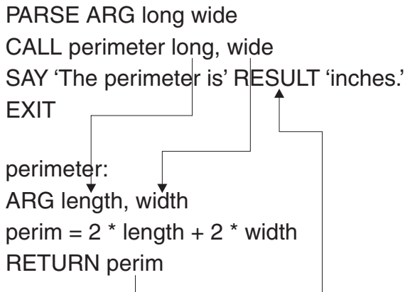
Figure 39. Example of Passing Arguments on the CALL Instruction
