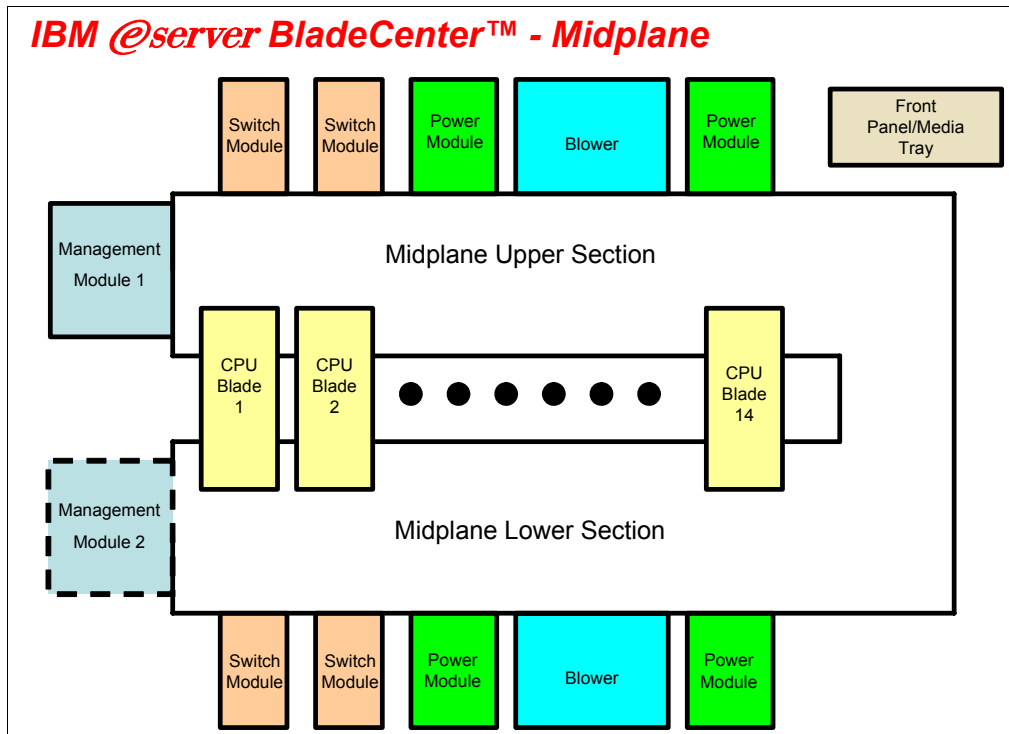
Figure 2-2 Midplane view
