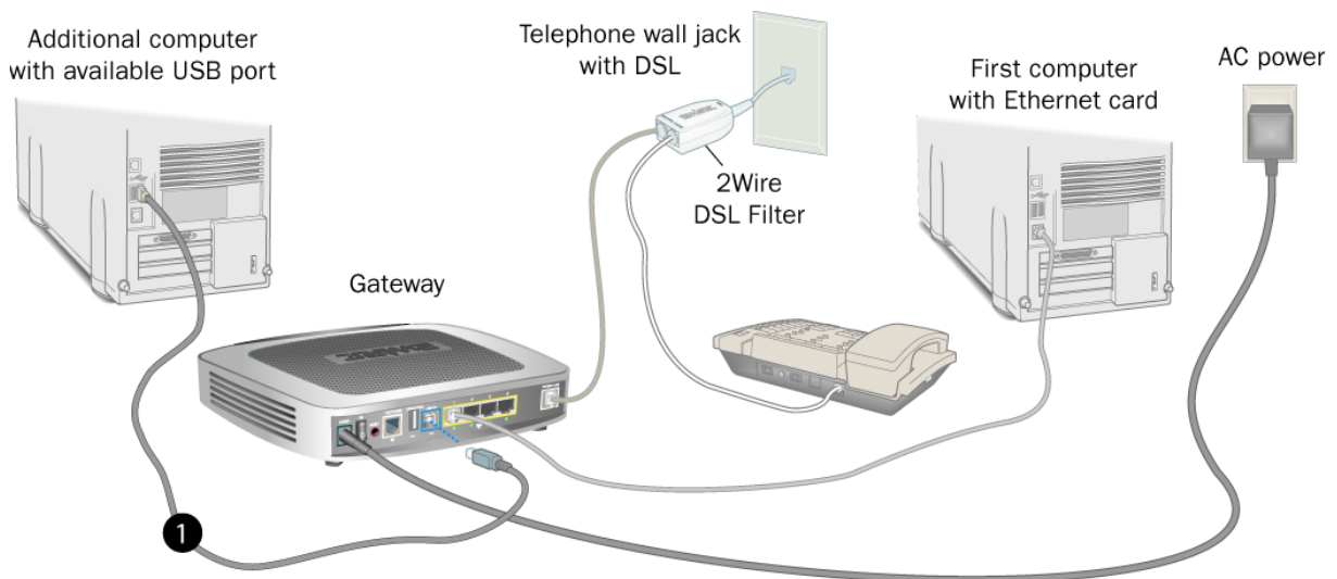
Figure 5. Gateway Connected to Second Computer Via USB
