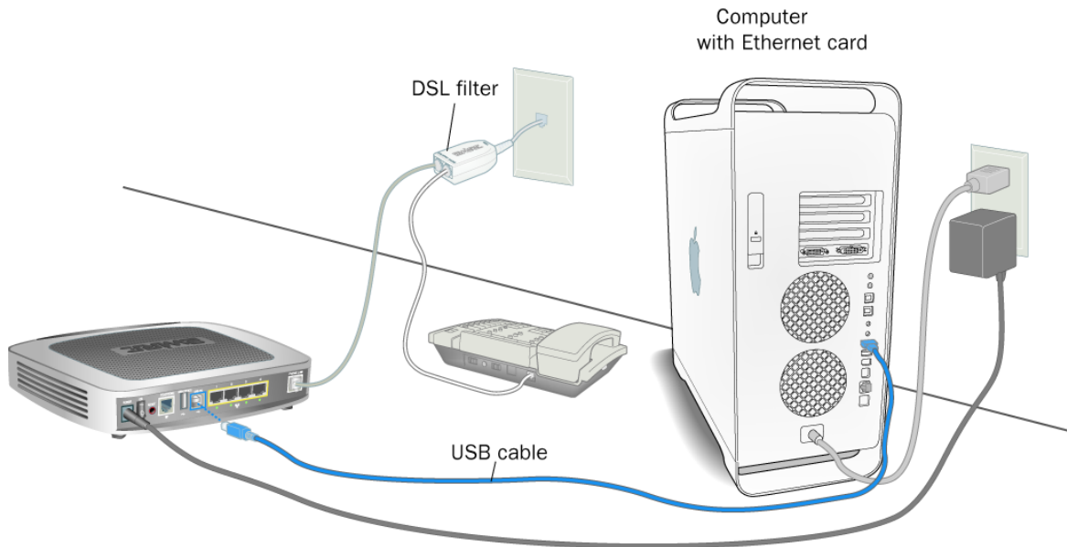
Figure 8. Gateway Connected Via USB (Macintosh)
