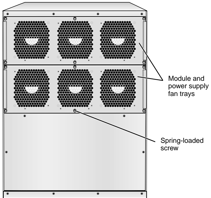
Figure 1 Location of FanTrays in the Rear of the Switch 4007R 8-slot Chassis
