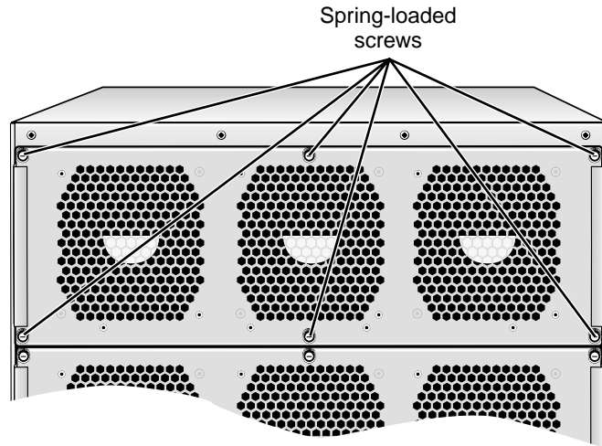
Figure 2 Location of the Six Fan Tray Spring-loaded Screws
