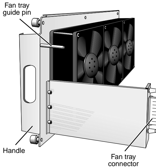
Figure 4 Fan Tray Connector and Guide Pin
