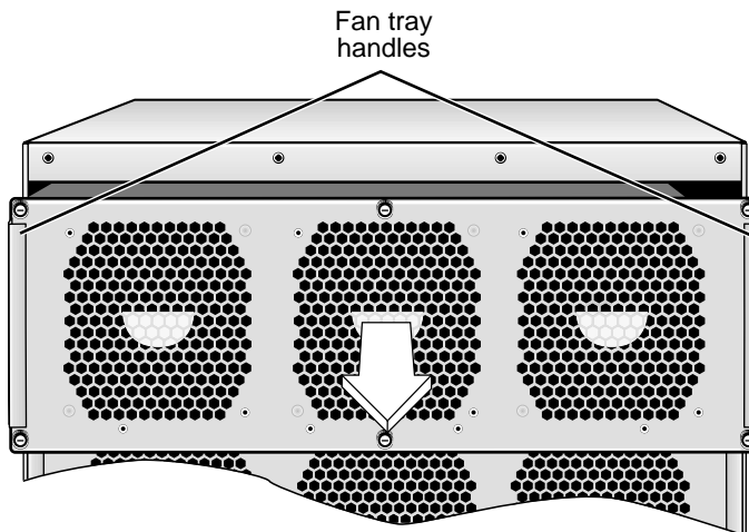
Figure 3 Removing the Fan Tray Using the Handles
