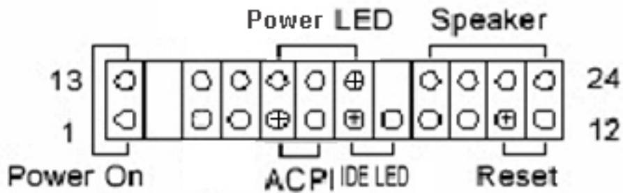
JANEL1: Front Panel Connector Pin Assignments
