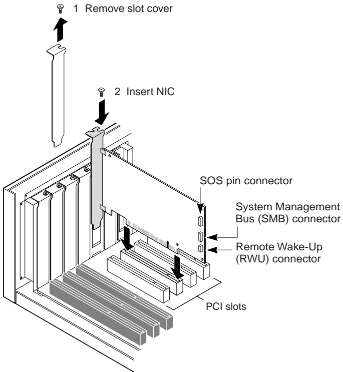
Figure 1 Installing the NIC
