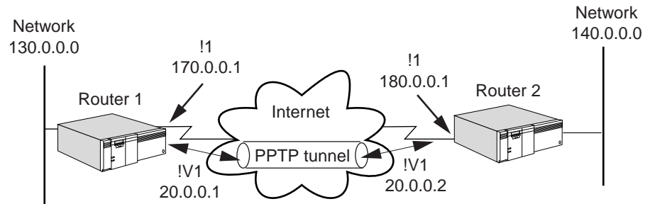
Figure 1 VPN PPTP Tunnel
