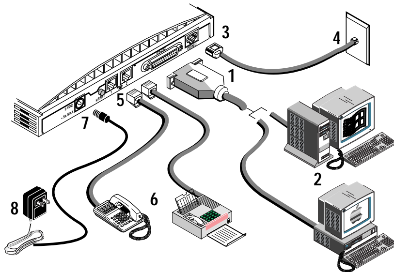
Figure 1 Installation Diagram
