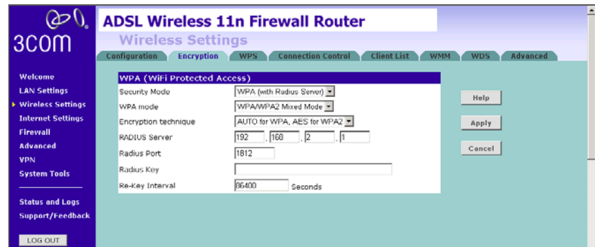
Figure 49 WPA (with RADIUS Server) Screen
